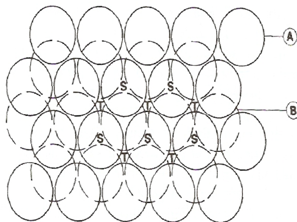
Fig. 1.13 Two cp layers arranged in A and B positions. The B layer occupies the P positions of Fig. 1.12
