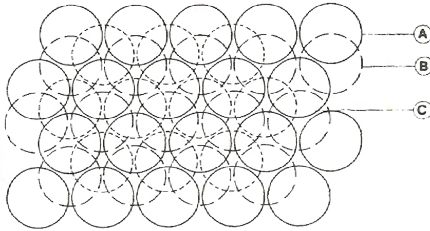
Fig. 1.14 Three close packed layers in ccp sequence
