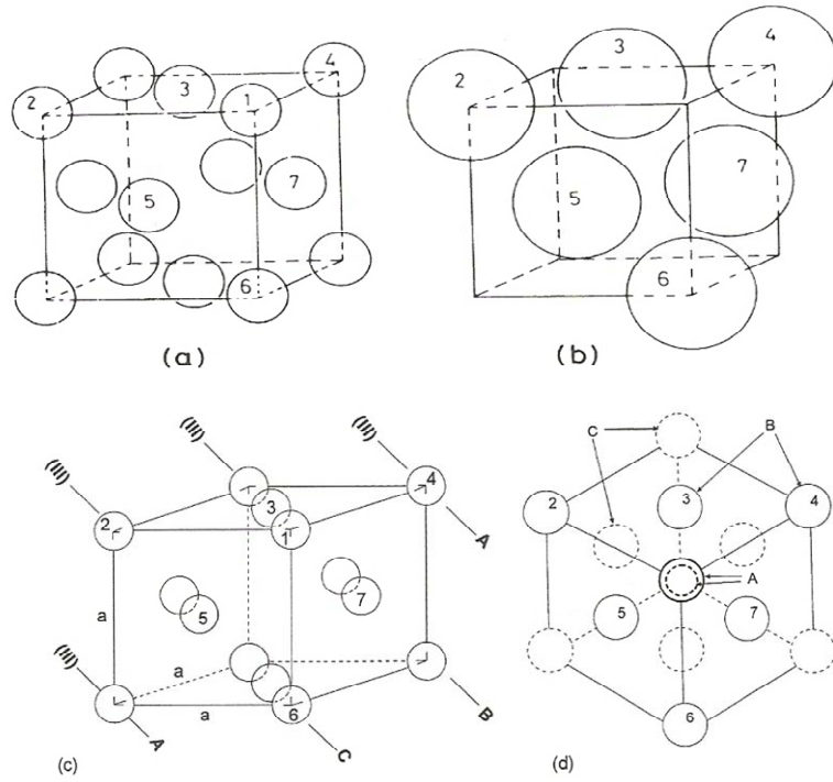
Fig. 1.16 Face centred cubic unit cell of a ccp arrangement of spheres
