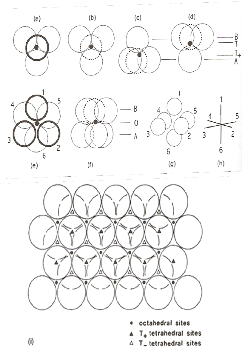
Fig. 1.19 Tetrahedral and octahedral sites between two close packed anion layers, seen from different perspectives. (a, b) Projection down threefold axis of T_+ , T_- sites. (c, d) Tetrahedral sites edge-on. (e) Projection down threefold axis of octahedral site and (f) seen edge on. (g, h) Conventional representation of octahedral site. (i) Distribution of T_+ , T_- , O sites between two cp layers
