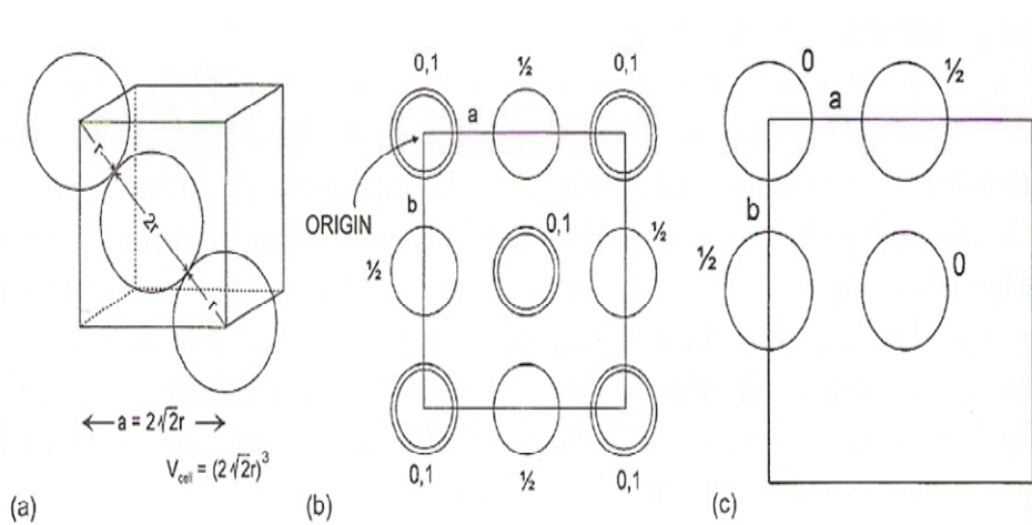
Fig. 1.18 (a) Unit cell dimensions for a face centred cubic unit cell with spheres of radius, r in contact along face diagonals. (b,c) Projection of a face centred cubic structure onto a unit cell face
