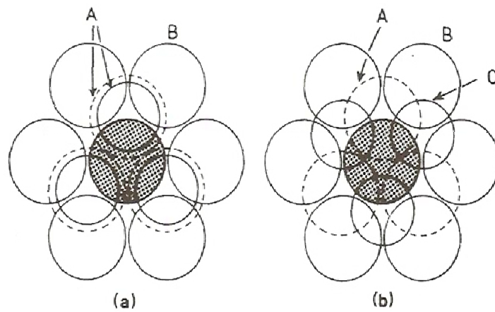
Fig. 1.15 Coordination number 12 of shaded sphere in (a) hcp and (b) ccp structures. The shaded sphere is in the B layer, the layer underneath is A and the layer above is either (a) A or (b) C
